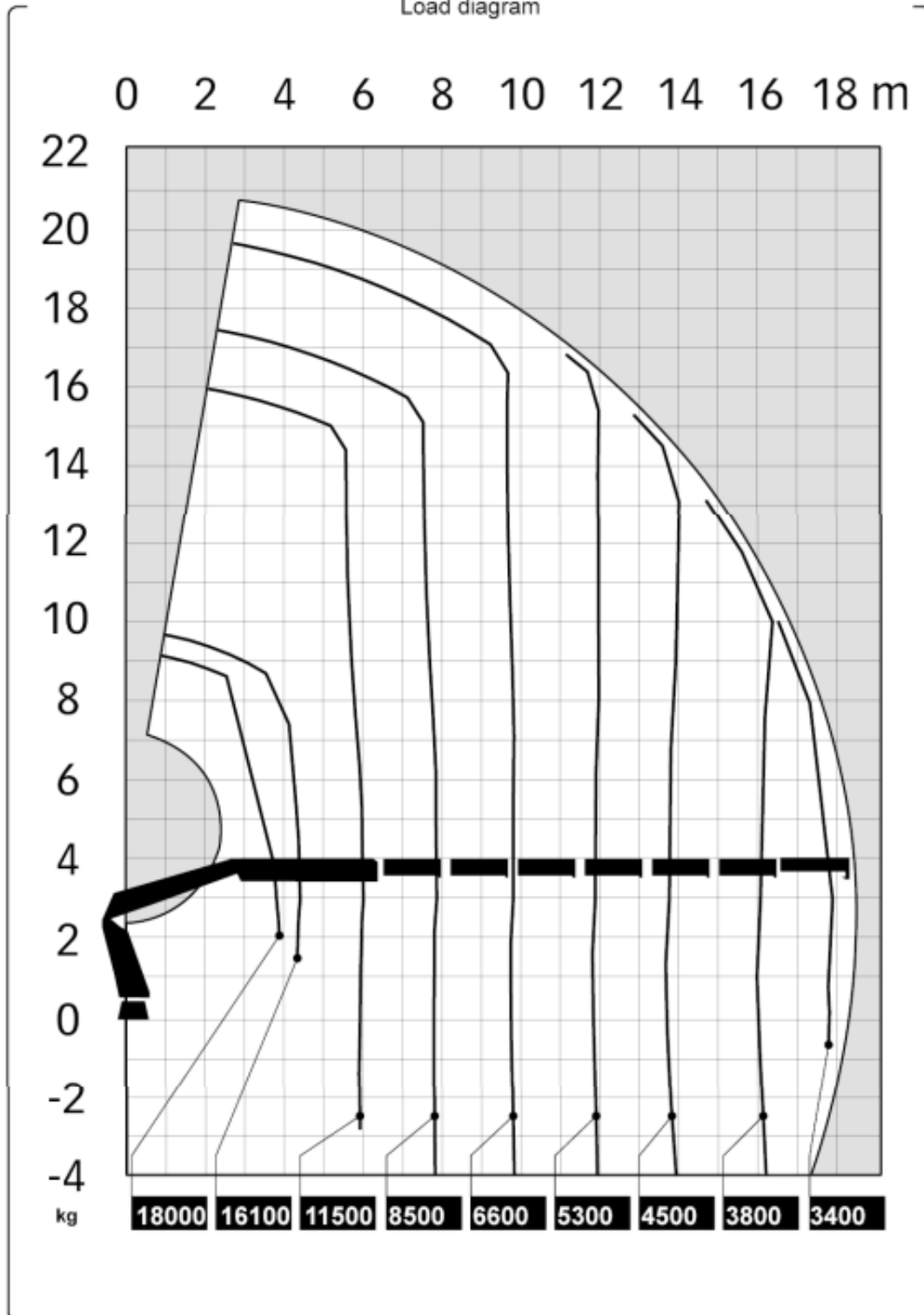
Load diagram
